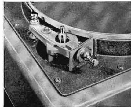
Unique Presto drive system. Step pulley on motor shaft drives against rubber tire on turntable rim. Lever changes speed instantly from 78 to 33 1/3 RPM.
