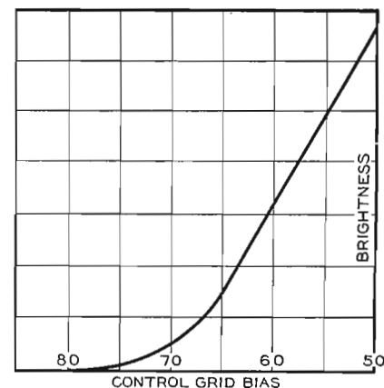
Fig. 2. The linear light voltage characteristic.
