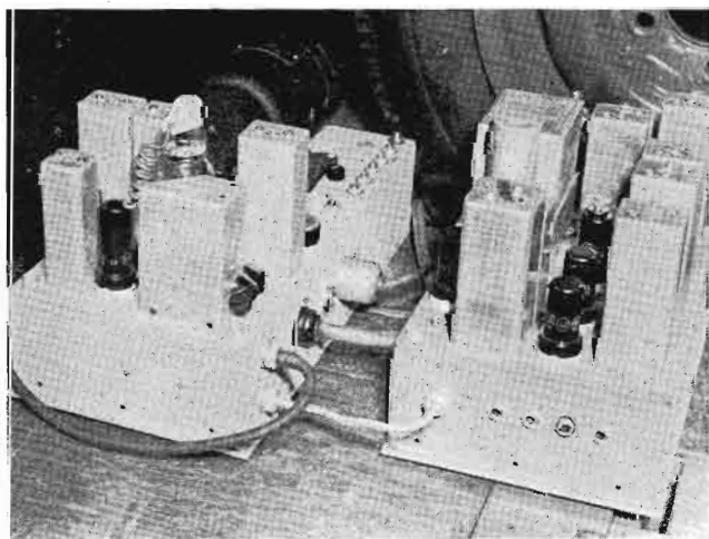
Left: Fig. 4. The General Electric mobile f-m police equipment.
